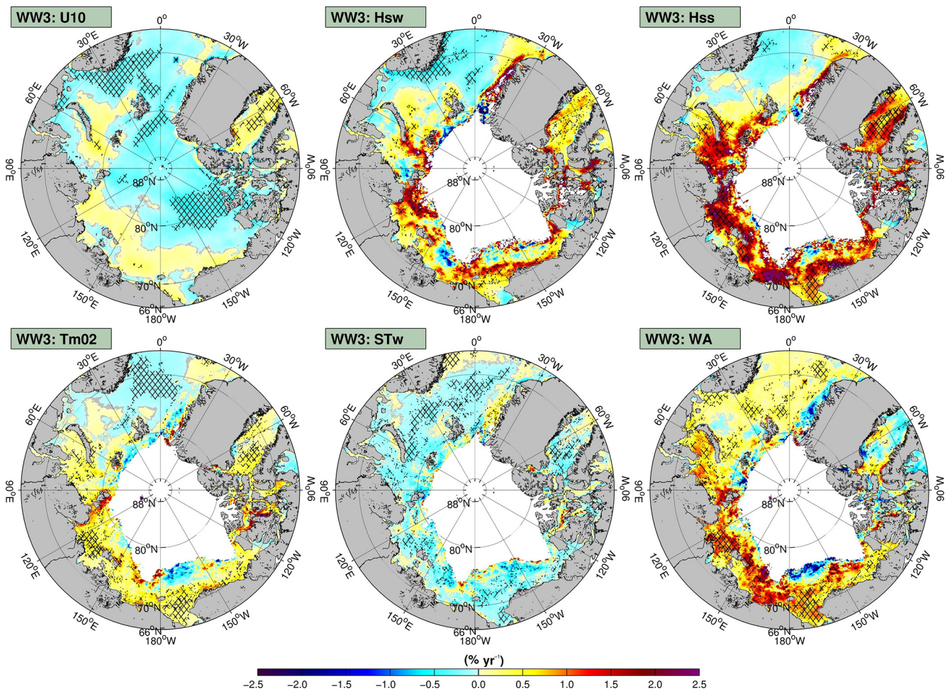
Figure 8. Sen’s slope with the Mann–Kendall test (thatched areas) for monthly averaged wind speeds (U10) (top left), wind-sea wave heights ( H_{sw} ) (top center), swell wave heights ( H_{ss} ) (top right), average wave period ( Tm02 ) (bottom left), wind-sea steepness ( ST_w ) (bottom center), and wave age (WA) (bottom right) from the wave hindcast in percentage per year relative to the average.
