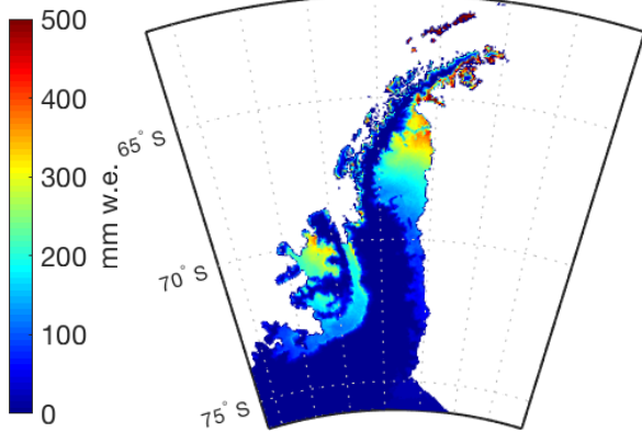
(a) RACMO mean melt
