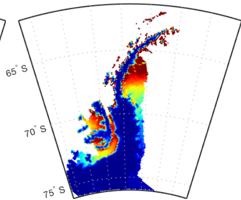
(b) MAR mean melt
