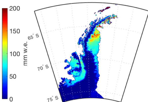
(c) RACMO SD melt
