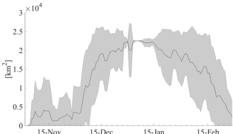
(g) QuikSCAT ft3 melt climatology
