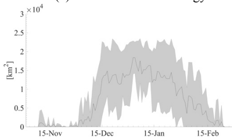
(a) MAR melt climatology
