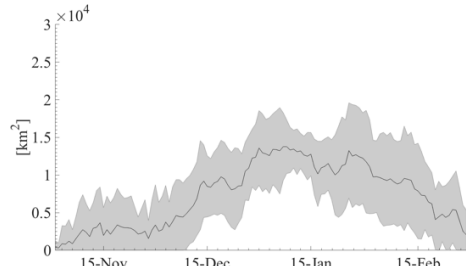
(a) MAR melt climatology
