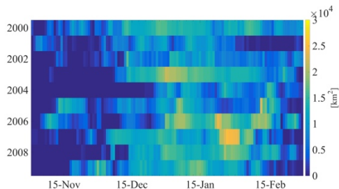
(b) MAR interannual
