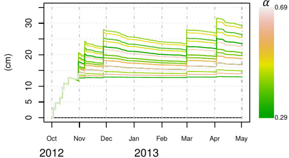
Snow depth time series at transect points
