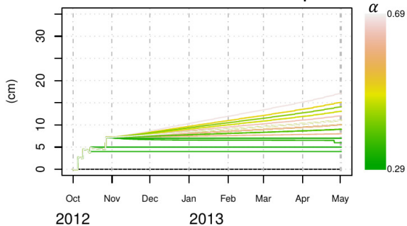
DH thickness time series at transect points
