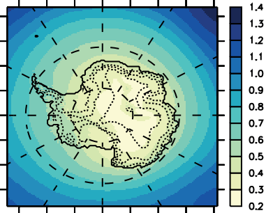
(a) Mean specific humidity (g kg -1 )
