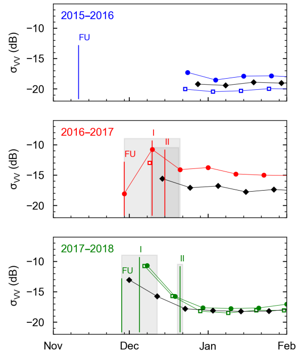
Figure 9. TerraSAR-X median VV backscattering is plotted versus time for each year (color coded). Three orbits are shown for orbits 13 (empty square), 21 (circle), and 89 (black diamond). The freeze-up date (FU, from time-lapse photography), the post-freeze-up peak (I, from TerraSAR-X), and the beginning of the monotone X band (II, from TerraSAR-X) are identified with vertical bars. Estimates for each indicator are indicated by shaded gray areas.
