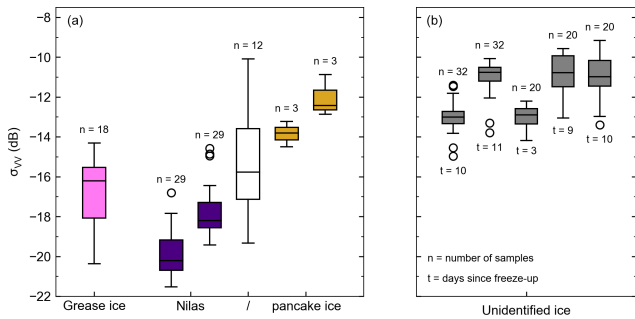
Figure 8. TerraSAR-X median VV backscattering values observed over AOIs of ice types identified from time-lapse photography in 2016 and 2017. The number of median values used ( n ) is written above each box. Outliers are plotted as empty white circles. (a) Grease ice (pink) was observed on the orbit 13 image from 26 November 2017. Nilas (dark purple) was observed on 28 and 29 November 2016 in orbits 13 and 21, respectively. A mix of nilas and pancake ice (white) was observed on 26 November 2017 in orbit 13. Pancake ice (yellow) was observed on 28 and 29 November 2016 in orbits 13 and 21. (b) Unidentified young ice (gray) was observed on 9 and 10 December 2016 in orbits 13 and 21, as well as on 1, 7 and 8 December 2017 in orbits 89, 13, and 21. The number of days since the freeze-up date ( t ) is written below each box.
