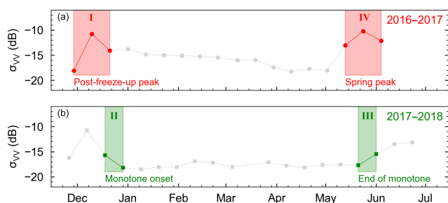
Figure 4. Examples of change detection in TerraSAR-X VV median backscattering. Peak detection for orbit 21 in 2016–2017 (a), and inflexion detection for orbit 13 in 2017–2018 (b). Derived indicators are the post-freeze-up peak (I), the beginning (II) and end (III) of the monotone period, and the spring peak (IV).
