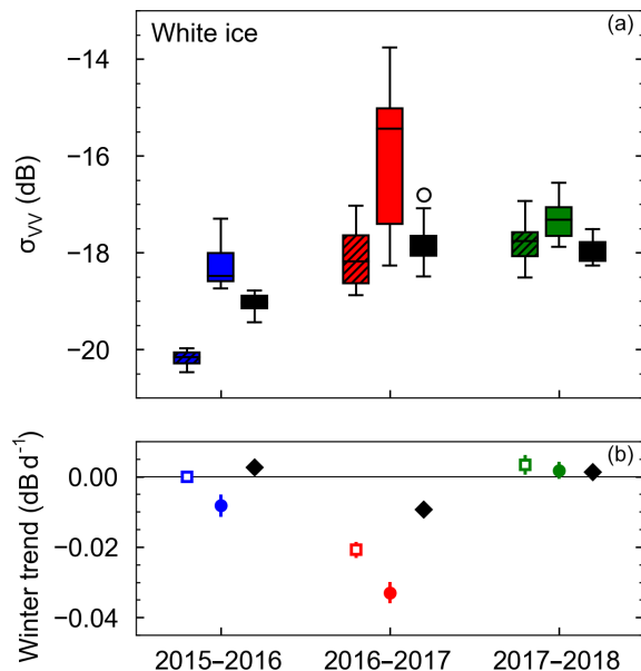
Figure 10. Characterization of TerraSAR-X VV winter backscattering. (a) Winter median by year (color coded) for orbits 13 (dashed, ascending, 17:32, 38°), 21 (solid, descending, 06:25, 40°), and 89 (black, ascending, 17:40, 46°). The seasonal median is computed from image medians, which were computed from AOI medians. Empty circle markers represent outliers. (b) Winter trend by year (color coded), for orbits 13 (empty square), 21 (circle), and 89 (black diamond). A horizontal black line indicates the point of zero trend. The trend is defined as the slope of the linear fit to the winter image medians (see Fig. S6). Error bars are the standard error associated with the fit.
