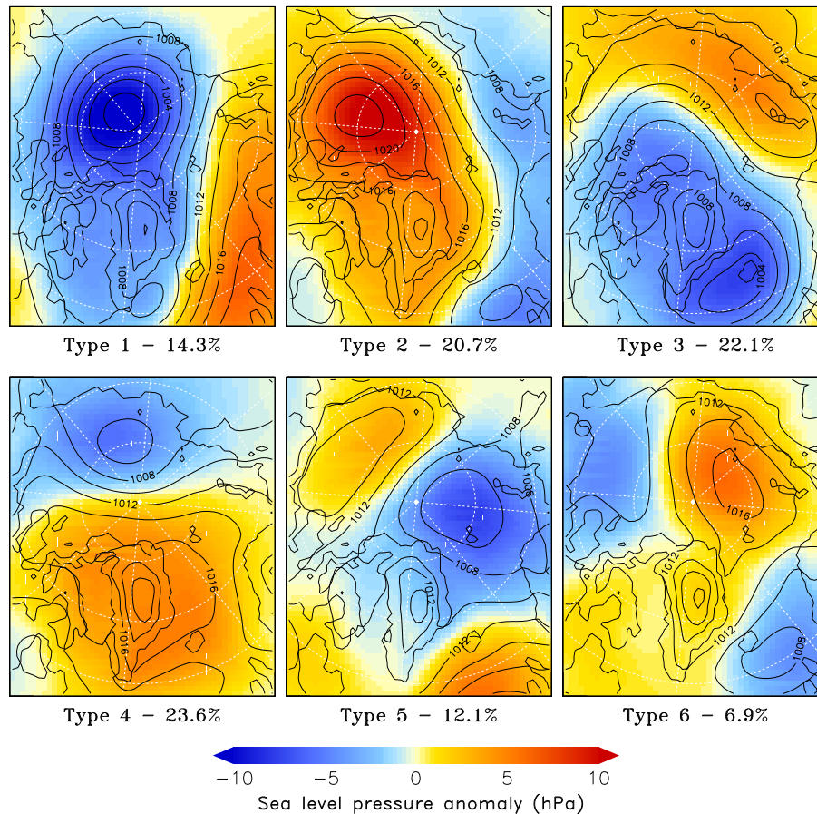
Figure 1. The SLP-based reference circulation types over the 1980–2012 (JJA) period for the ERA-Interim are represented by the solid black isobars (in hPa). The SLP anomaly (in colours) is calculated as the difference between the class mean SLP and the seasonal mean SLP over 1980–2012. The average frequency of each type is also given.
