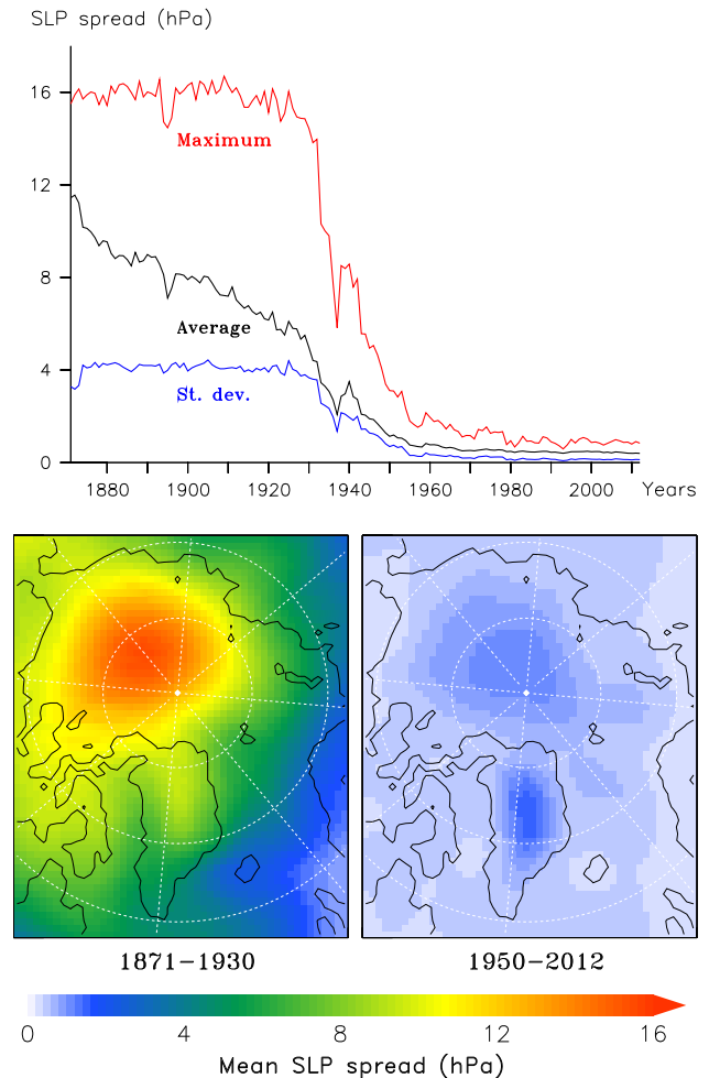
Figure 3. Top: the average SLP spread and its standard deviation are calculated as the seasonal (JJA) average 20CRv2 spread and its standard deviation over the oceanic pixels of our domain. The maximum SLP spread is the value of the oceanic pixel showing the highest seasonal (JJA) average spread of each year. Bottom: the SLP spread is calculated as the average 20CRv2 spread over the 1871–1930 summers (JJA), left, and over the 1950–2012 summers, right.
