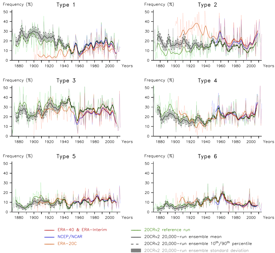
Figure 2. The dotted light lines represent the annual (JJA) SLP-based circulation type frequencies for ERA-Interim (1979–2014) and ERA-40 (1958–1978), NCEP/NCAR (1948–2014), ERA-20C (1900–2010), and the 20CRv2 reference run and the 20CRv2 20 000-run ensemble mean (1871–2012). The corresponding solid lines represent the 10-year binomial running mean frequencies. For the 20CRv2 20 000-run ensemble, the 10th and the 90th percentiles as well as the 1 standard deviation interval around the mean are also given.
