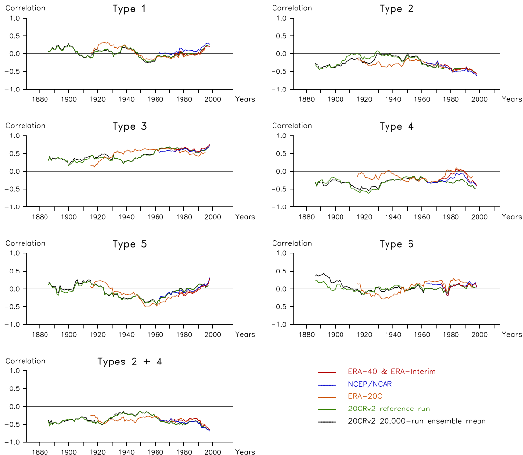
Figure 4. The 30-year running correlation is calculated between the annual (JJA) SLP-based frequencies of each type and the JJA CRU NAO index. For the “Types 2 + 4” correlation, the frequencies of types 2 and 4 have been summed before computing the correlation.
